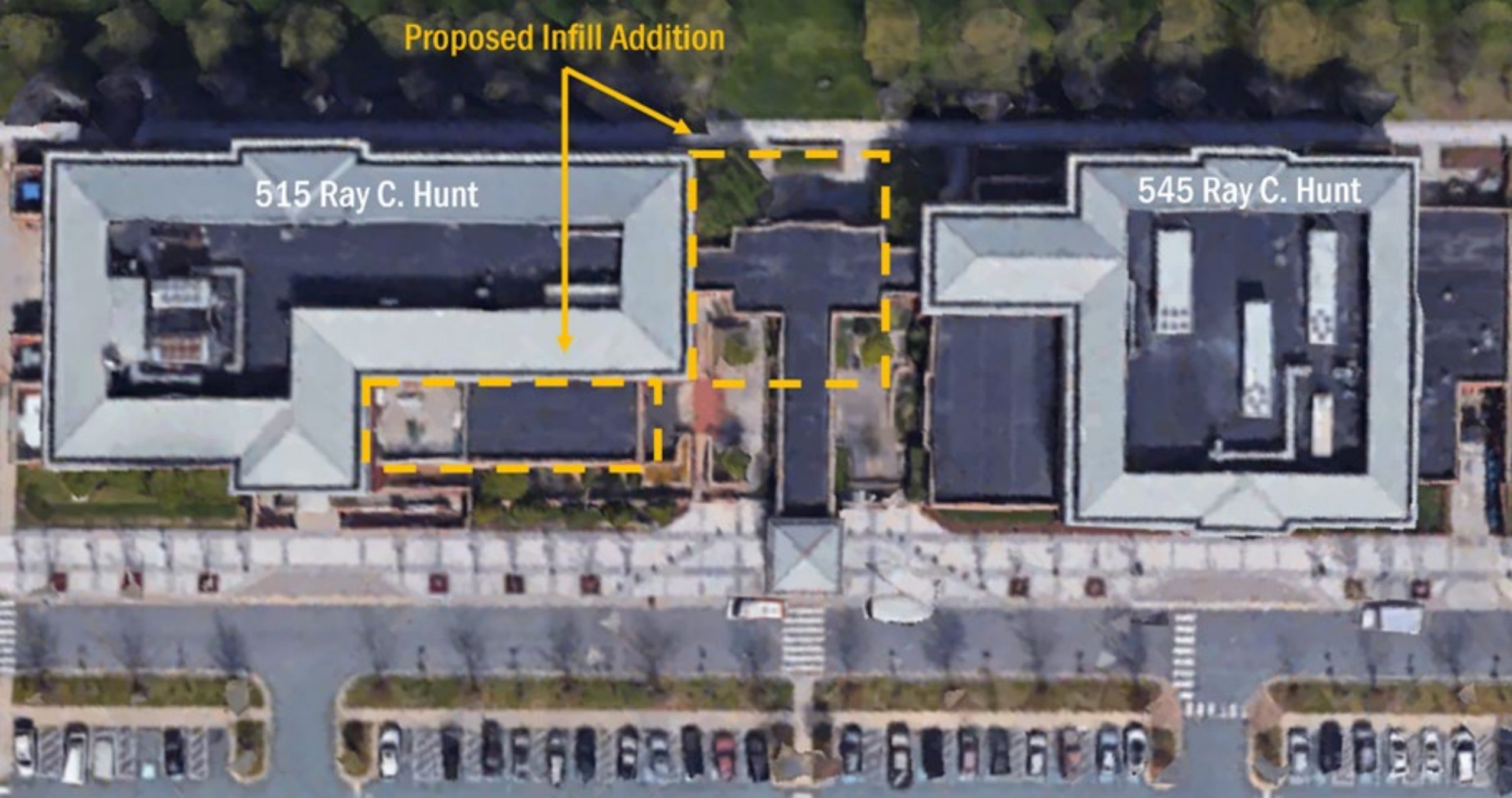
EXISTING SITE PLAN WITH PROPOSED ADDITIONS
